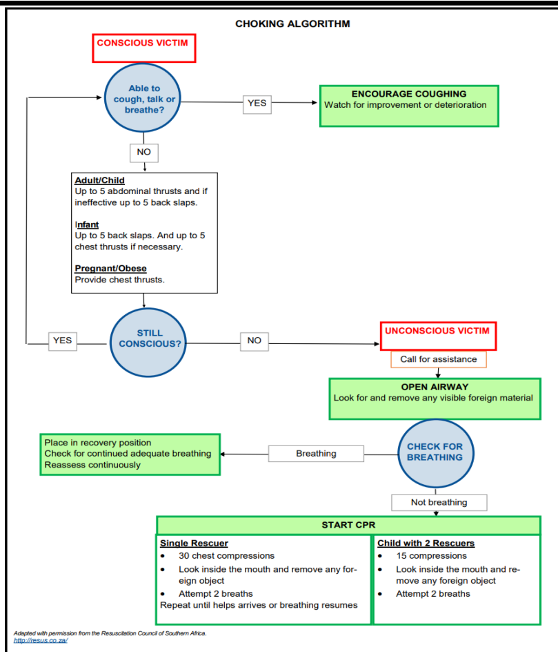
Figure 21.4 Choking algorithm
